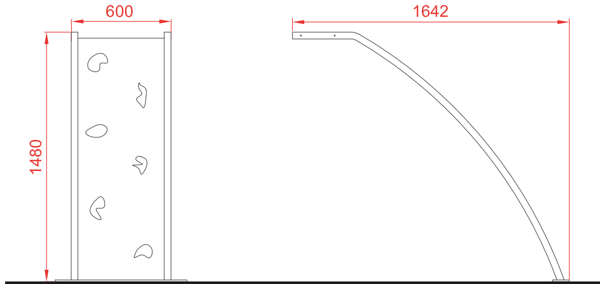
General dimensions (mm.)
