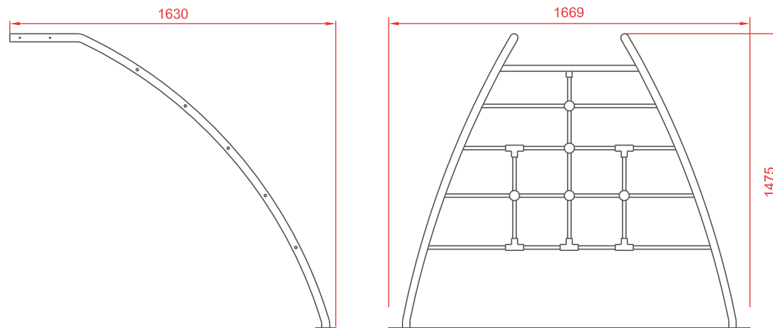
General dimensions (mm.)
